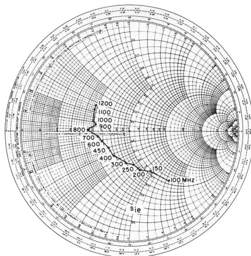
Smith-chart plot of input impedance for a 2N3563, common emitter configuration, from 100 to 1,200 MHz.
