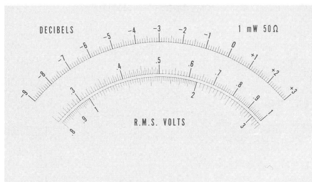
Linear dB scale available on Option 02 version of the 8405A.
