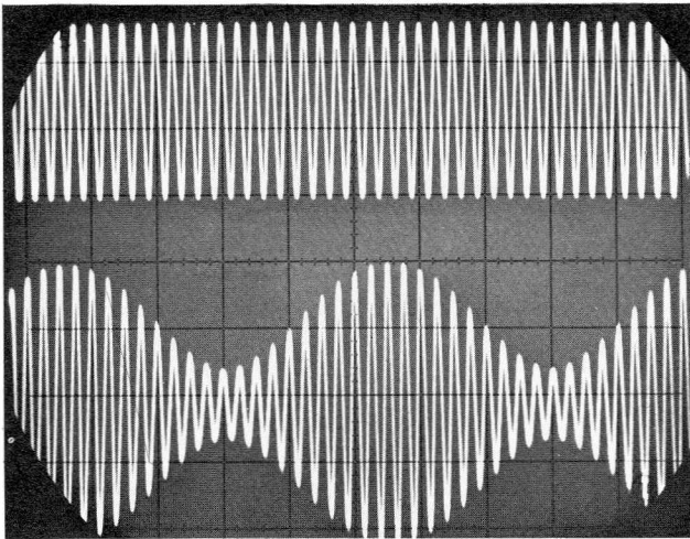
Reconstructed signal at 20 kHz IF Output. Input signal: 125 MHz CW (upper trace); 125 MHz CW with 1,000 Hz, 60% AM (lower trace).
