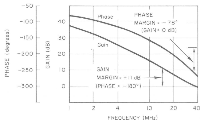
Open-loop gain and phase shift of a negative-feedback amplifier. As data indicates, amplifier is unstable.
